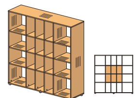
48H904 1588x430x1592
