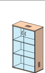
ШС44 740X372X1196
