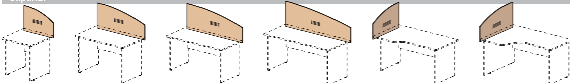
29P011 680X16x500 29P014 1100X16x500 29P015 1380X16x500 29P016 1600X16x500 29P012 800X16x500 29P013 1000X16x500
