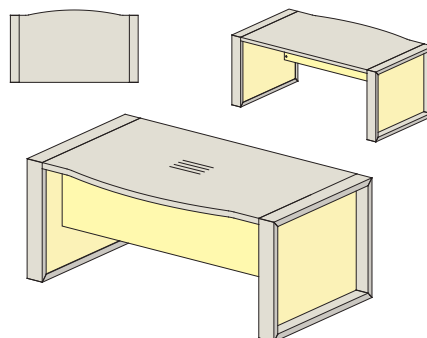
81S002 1800x1025x753
